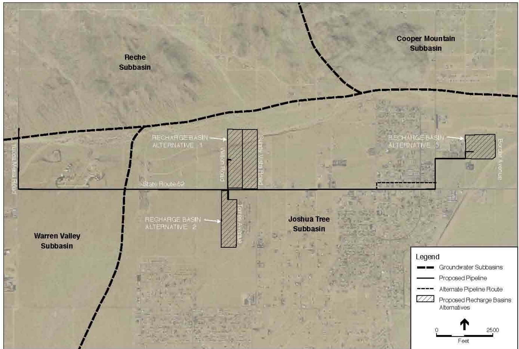
Figure 3.8-1 Groundwater Subbasins
