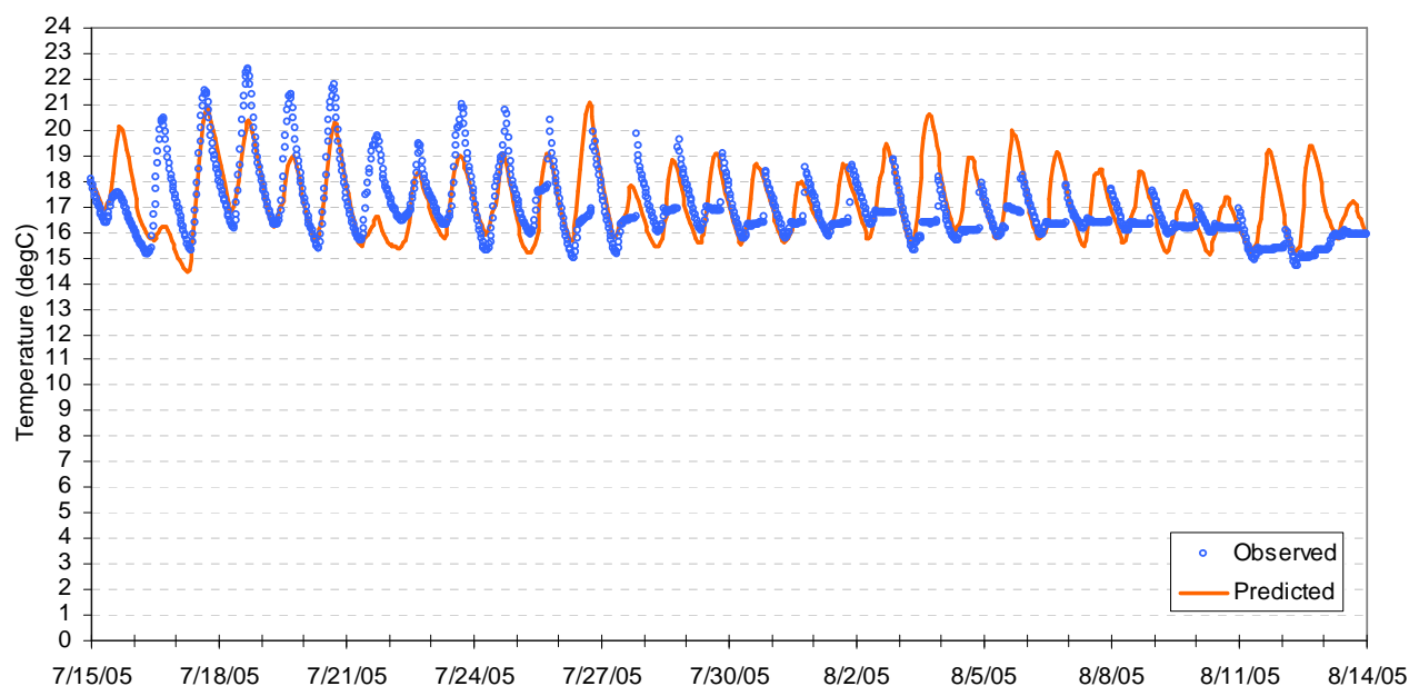
Figure 5. Modeled and observed hourly temperatures for Williams Creek
