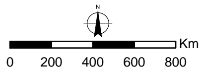
Albers Equal Area Projection
