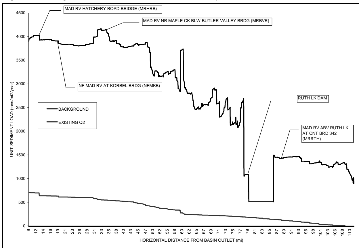
Figure 10. Longitudinal Plot of Unit Sediment Delivery for the Mad River
