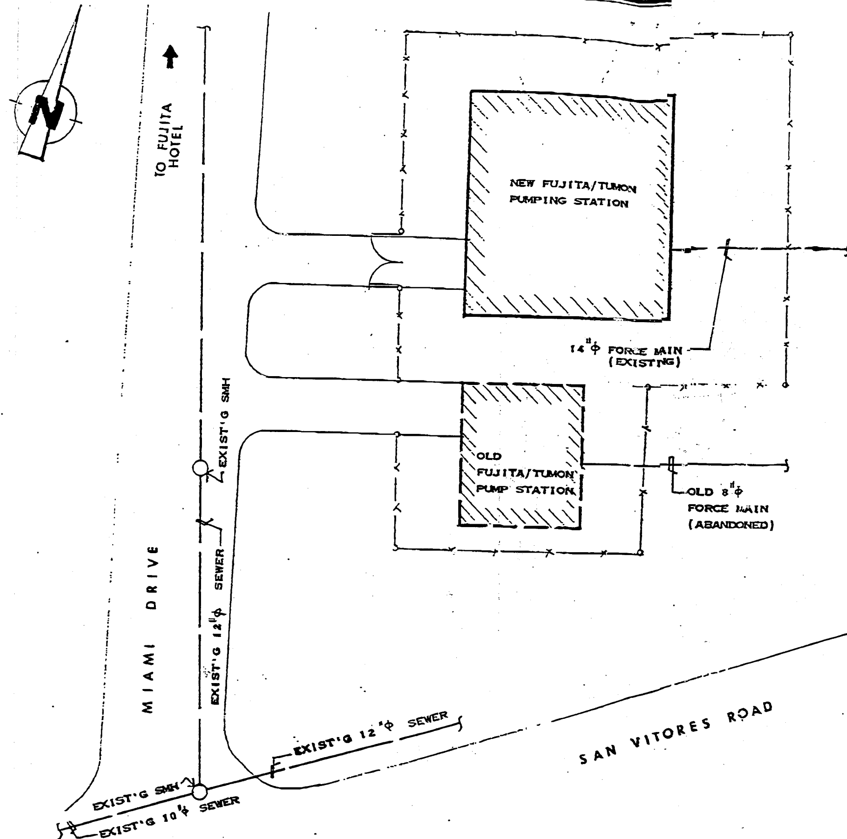
FIGURE 3 SITE PLAN- FUJITA PUMP STATION
