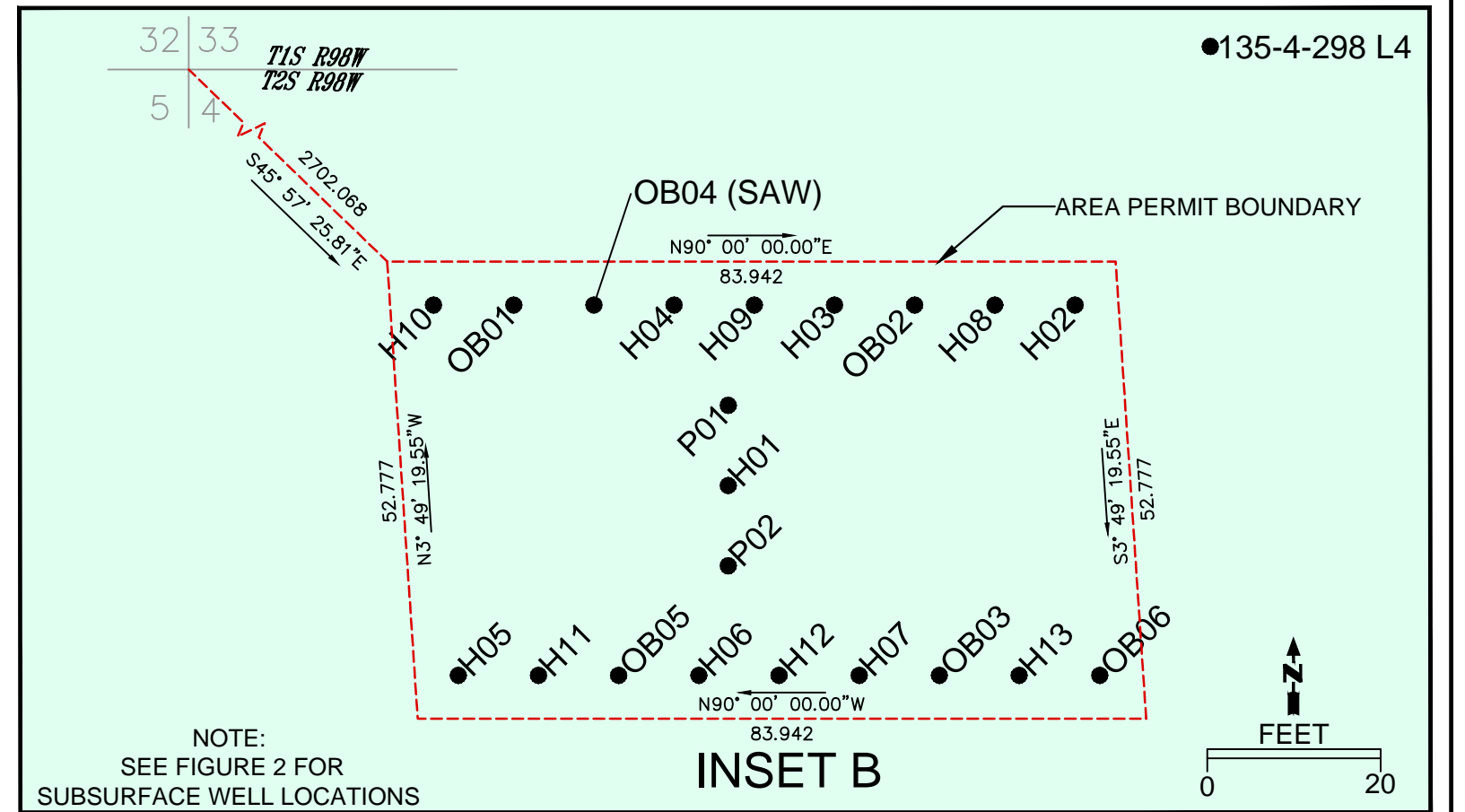
FIGURE 1 WELLS IN THE AREA OF REVIEW AND THE AREA PERMIT BOUNDARY
