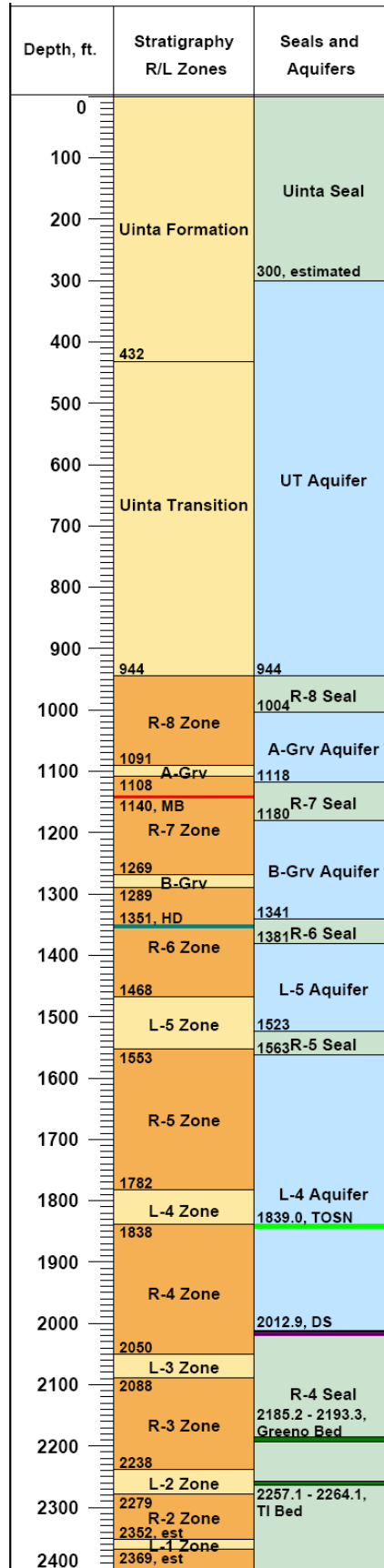
FIGURE 3 EAST RDD STRATIGRAPHY AND HYDROSTRATIGRAPHY
