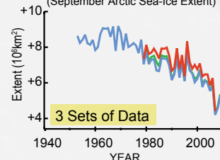
Sea-Ice ↓
