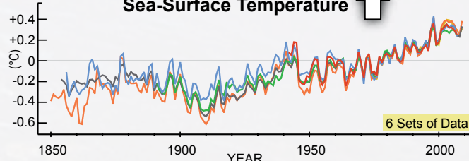
Sea-Surface Temperature ↑
