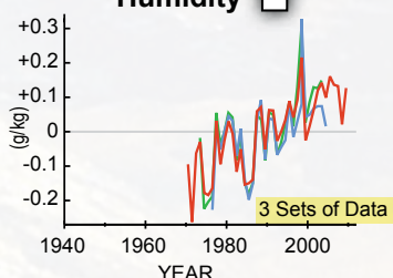
Specific Humidity ↑
