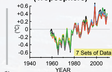
Air Temperature Near Surface (Troposphere) ↑
