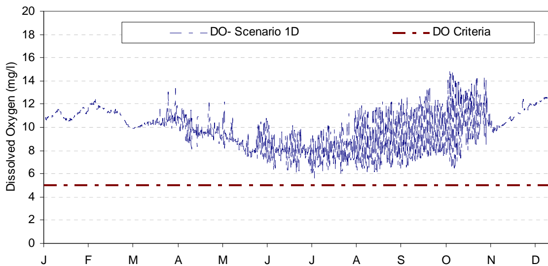
Figure 5-2. Dissolved oxygen standard compliance – Lost River at Stateline Road (LRSR).
