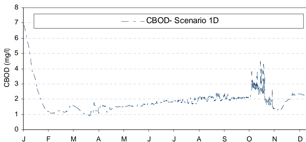
Figure 5-9. CBOD concentrations – Lost River at Stateline Road (LRSR).
