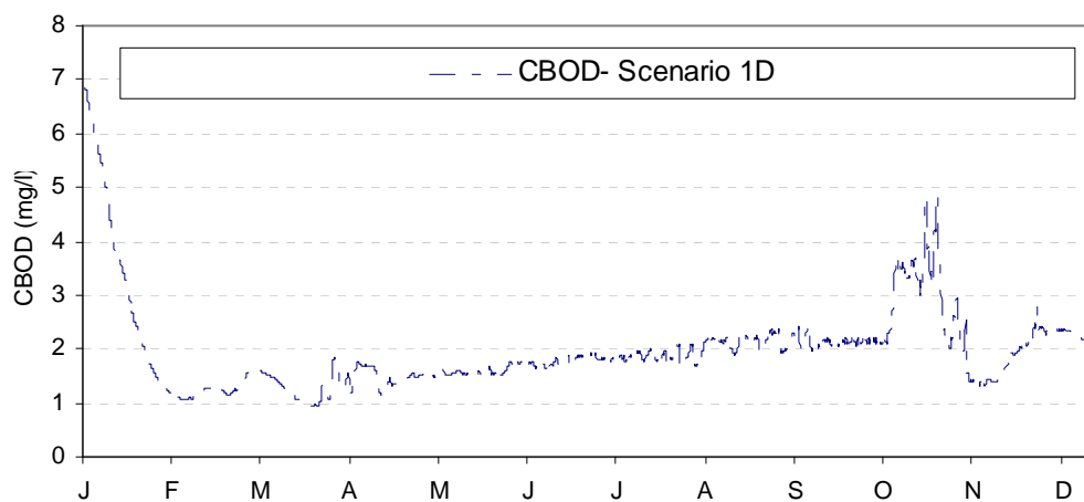
Figure 5-8. CBOD concentrations – Lost River at East-West Road.
