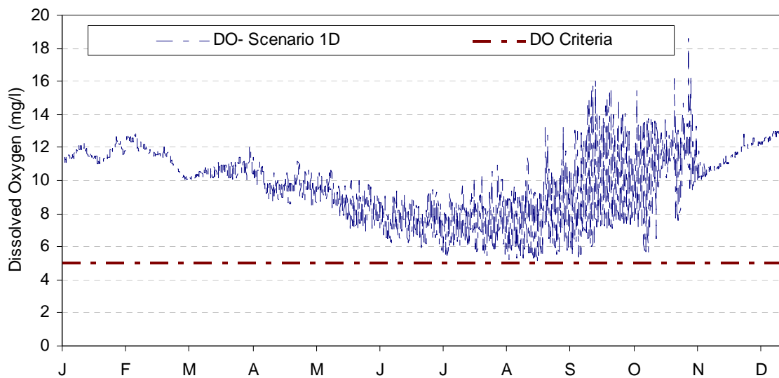
Figure 5-3. Dissolved oxygen standard compliance – Lost River at East- West Road (LREW).
