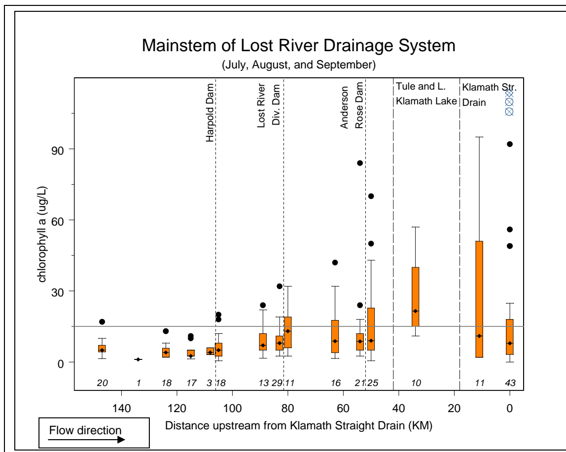
Figure 2-8. Longitudinal trends for Chlorophyll a during the critical summer months.
