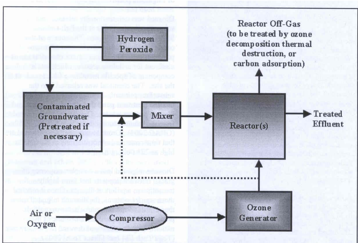
Exhibit 1: Process Flow Diagram of a Typical Ozone/Hydrogen Peroxide Groundwater Treatment System
