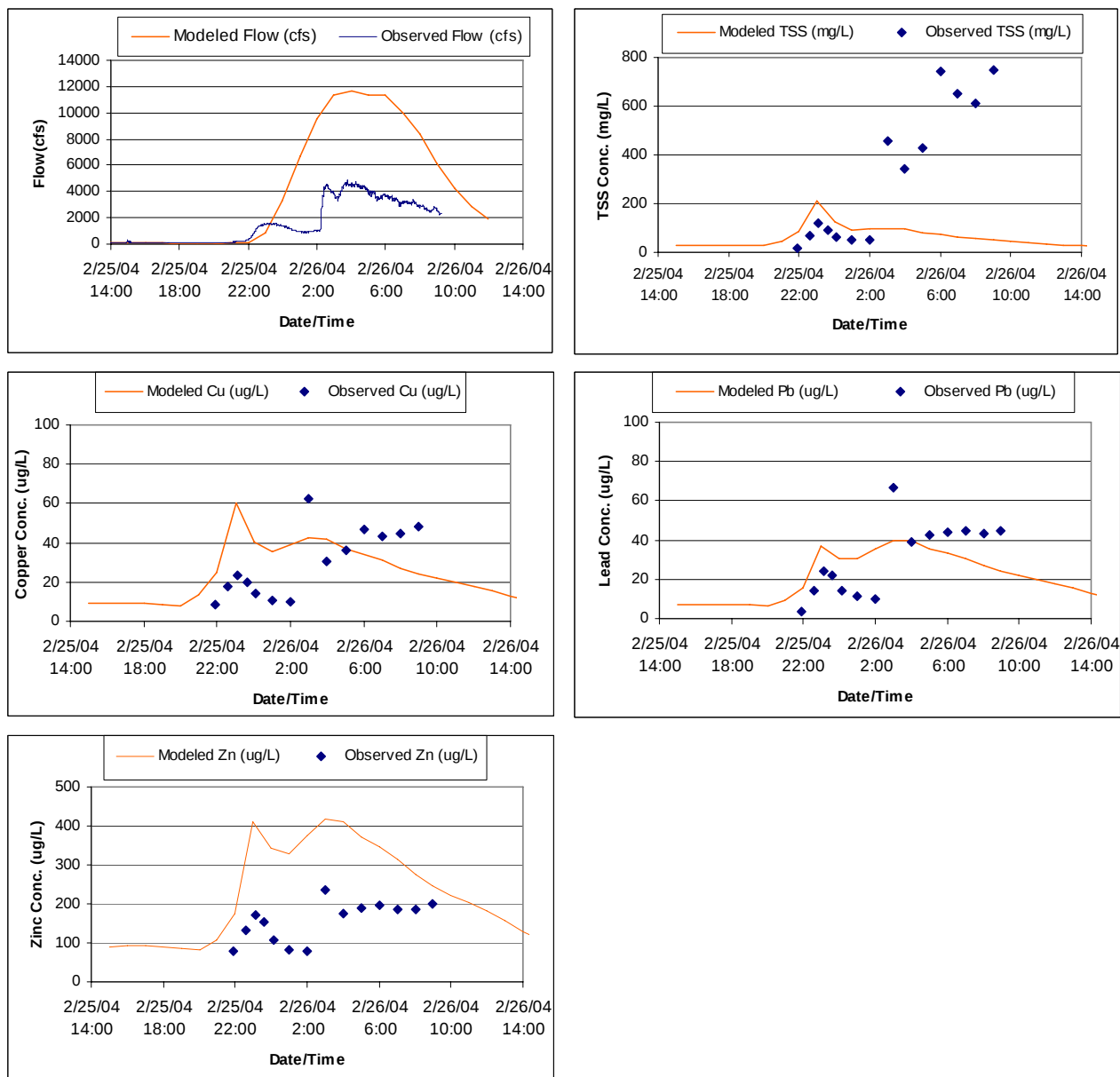
Figure C-2. Comparison of modeled and observed hydrology, TSS, copper, lead, and zinc at Coyote Creek for the February 25, 2004 storm event
