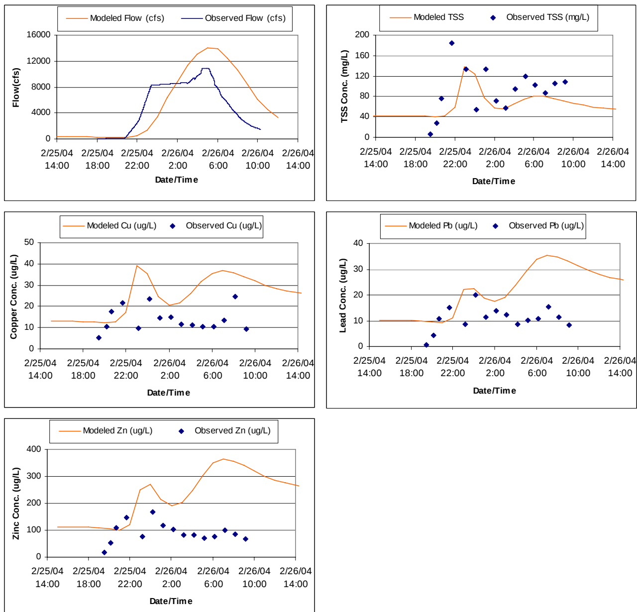
Figure C-1. Comparison of modeled and observed hydrology, TSS, copper, lead, and zinc at San Gabriel River for the February 25, 2004 storm event
