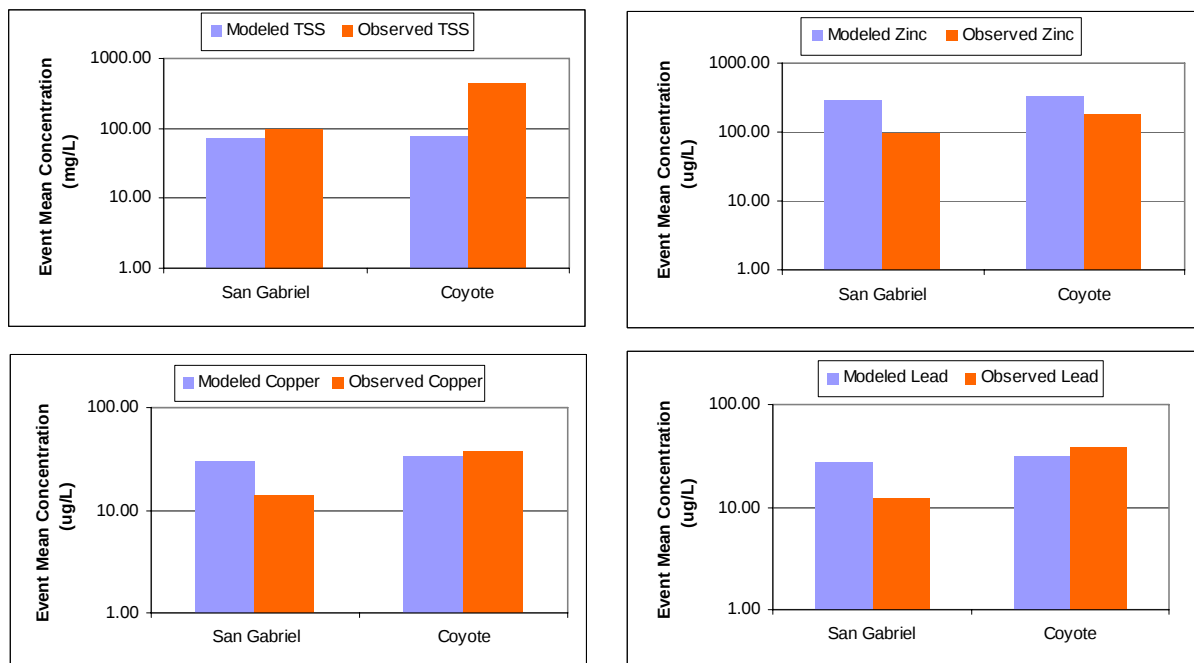
Figure C-3. Modeled and observed event mean concentrations for the February 25, 2004 storm event
