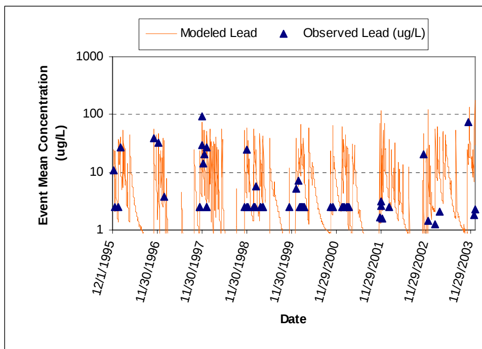
Figure D-7. Time series comparison of modeled and observed lead for the Coyote Creek
