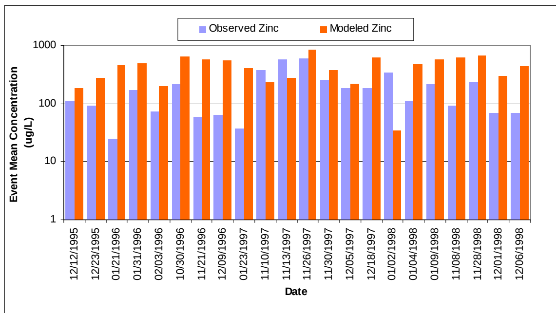
Figure D-30. Modeled and observed zinc event mean concentrations for the Coyote Creek from 1995 through 1998
