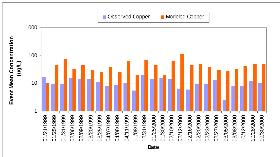
Figure D-25. Modeled and observed copper event mean concentrations for the Coyote Creek from 1999 through 2000
