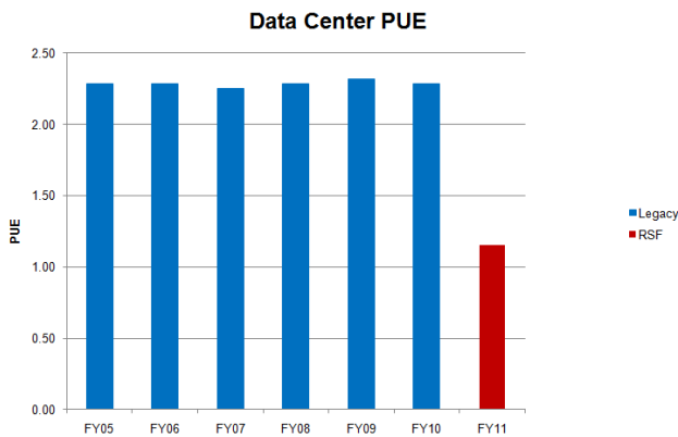
Figure 6. Energy requirements comparison of NREL's RSF data center to the legacy data
