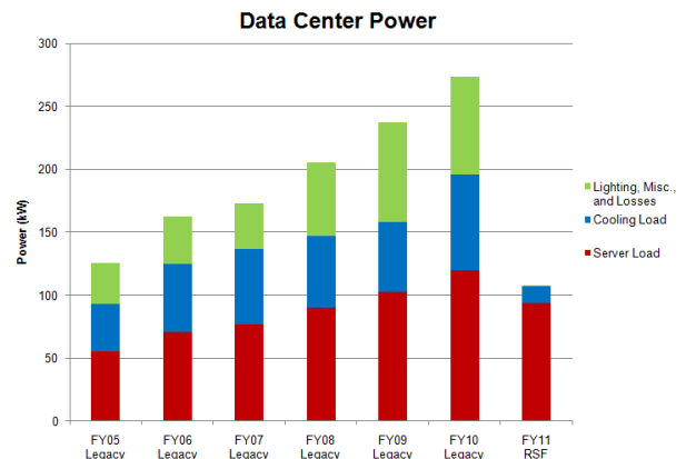
Figure 7. PUE comparison of NREL's RSF data center to the legacy data center.
