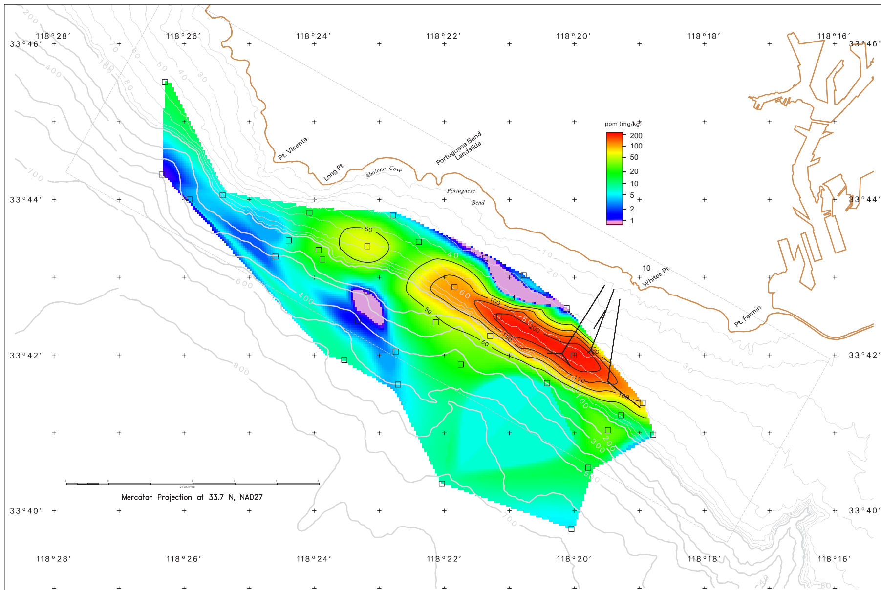
Figure 2. Peak Total DDT Determined Over a 4-cm Increment (taken from Lee (1994) Figure 34)
