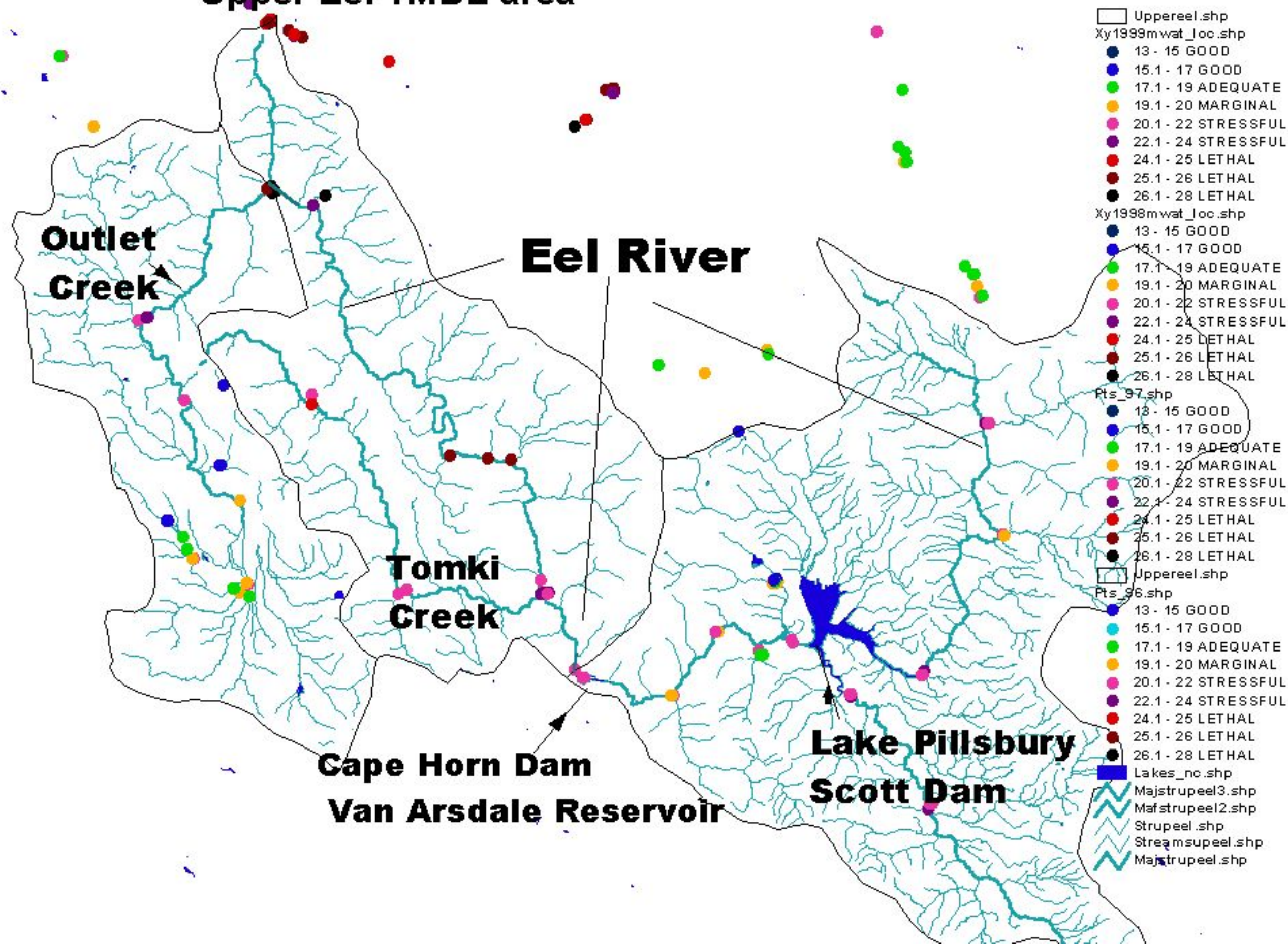
Figure 3: Stream Temperature Monitoring Upper Eel TMDL area
