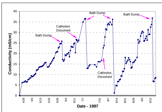
Figure 4. Conductivity Measurements in Rinse 1
