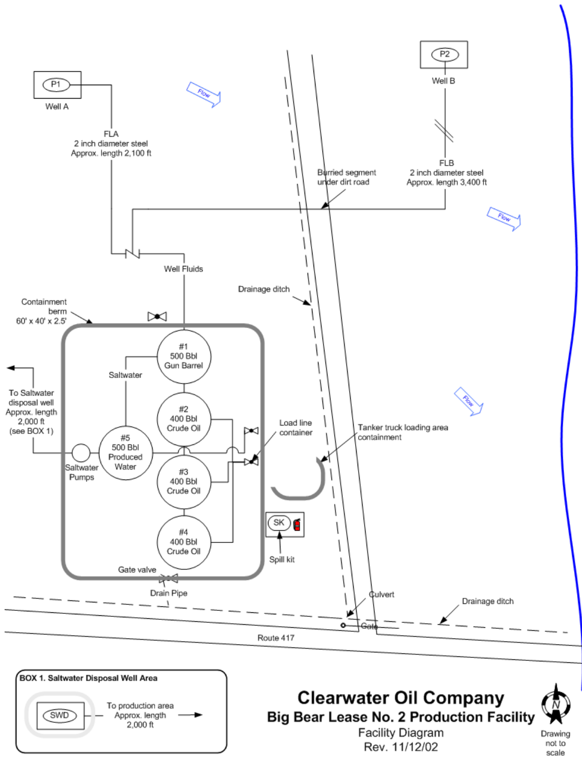
Figure A-2: Production Facility Diagram.
