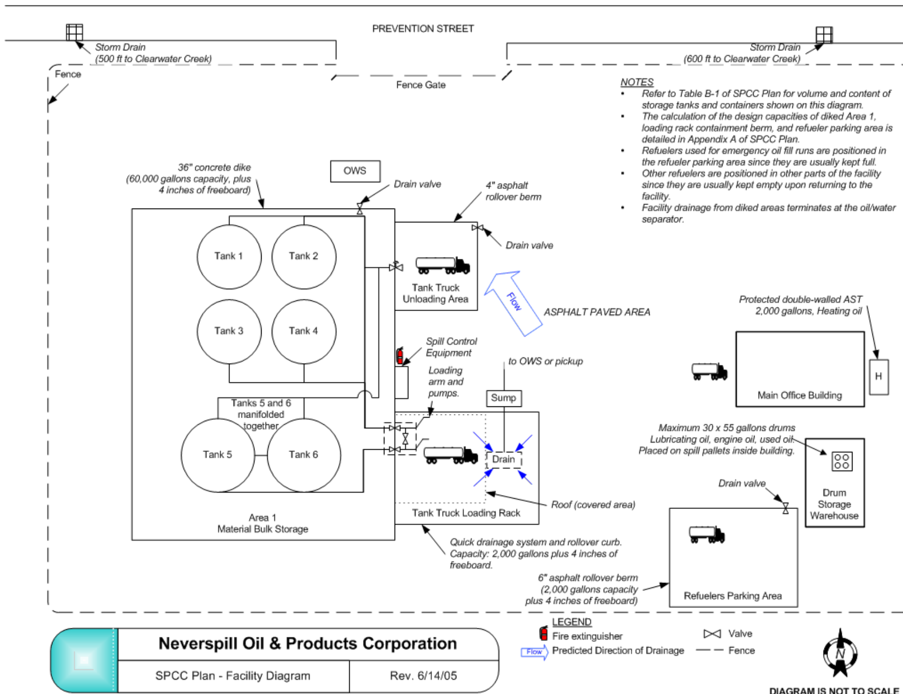
Figure 6-3. Example facility diagram, including loading and unloading areas.
