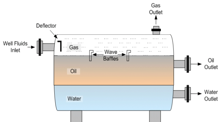
Figure 5-4. Low pressure free-water knockout.
