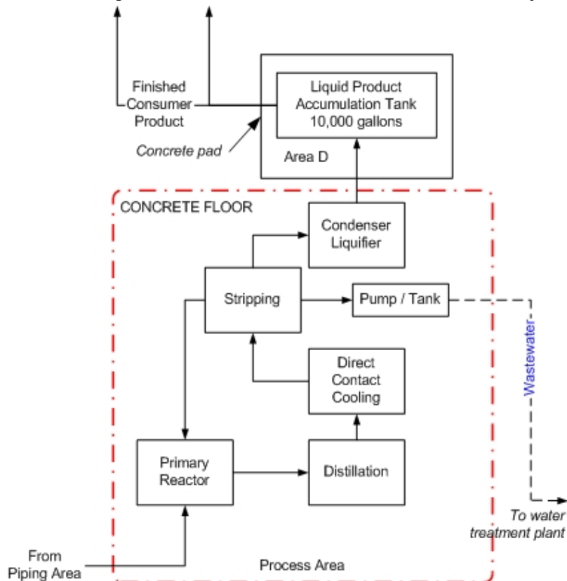
Figure 6-1. Example showing how manufacturing equipment could be represented in a facility diagram. Note that more detailed diagrams would need to be available at the facility.
