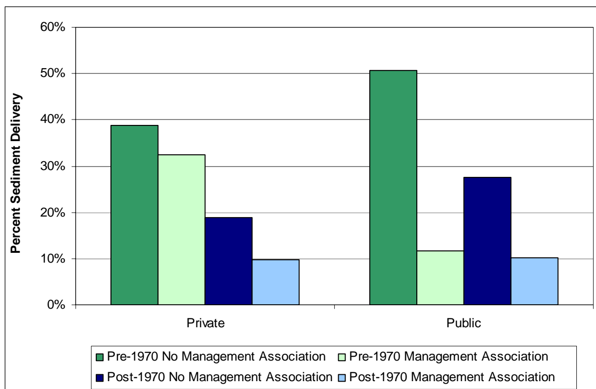
Figure 7. Percent sediment delivery by management association and time period
